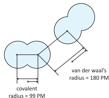
Covalent and van der Waal's radii of chlorine
